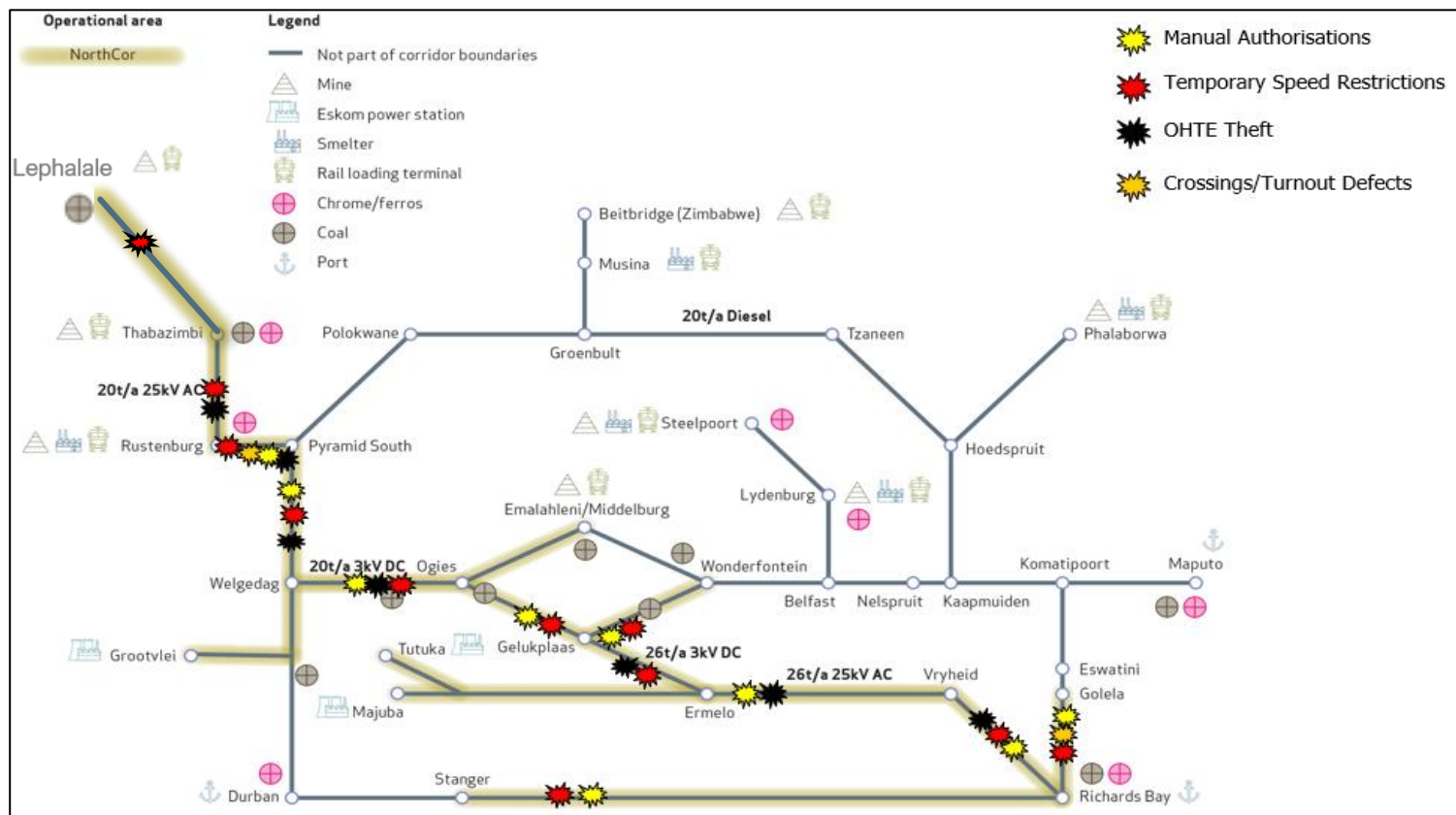
Figure 7: Network Condition for North Corridor (Source: Transnet)
