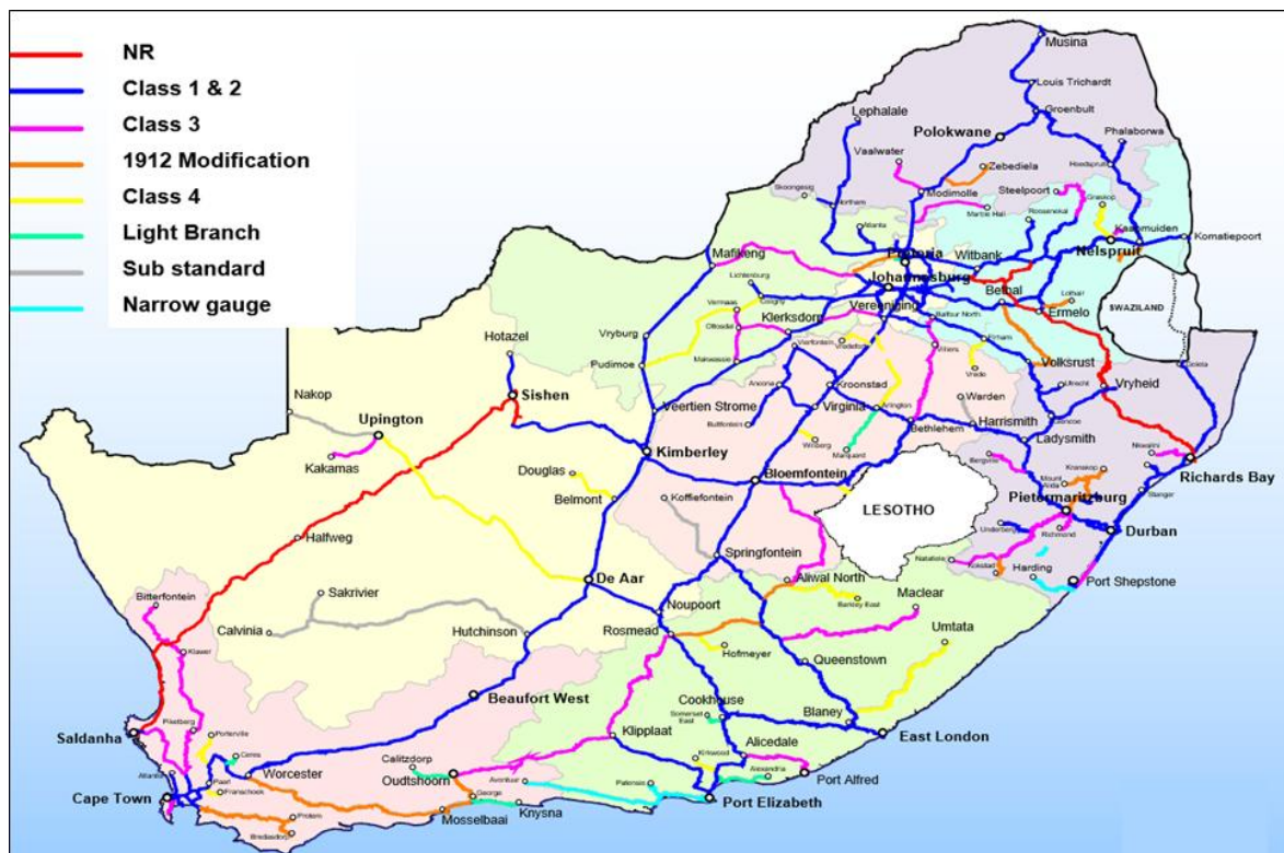
Classification of Railway Lines (Source: Transnet)
