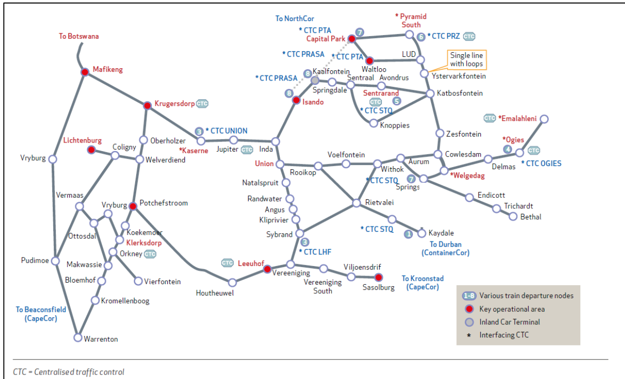
Figure 19: Central Corridor key lines
