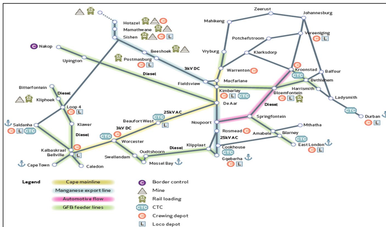
Figure 15: Cape Corridor key lines
